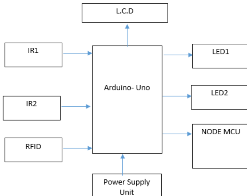
Fig1: Proposed block diagram
